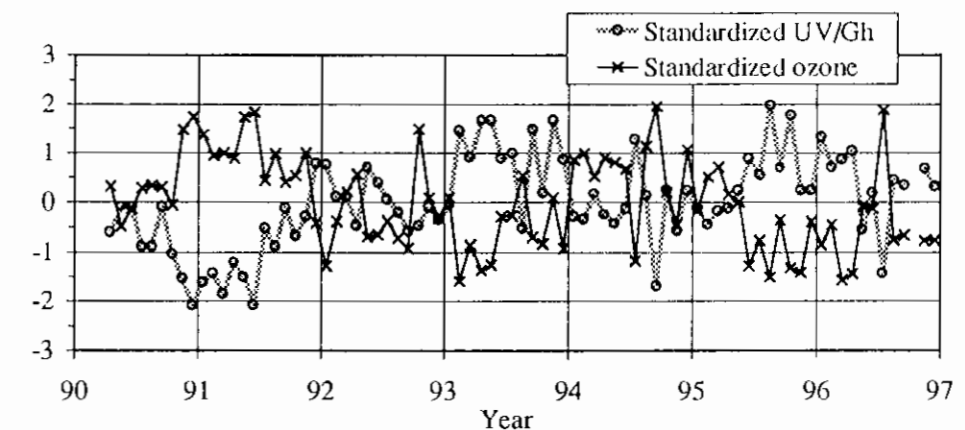
Figure 6.1 Standardized monthly values of total ozone and standardized monthly ratio between ultraviolet and global radiation for Norrköping 1990-1996.
