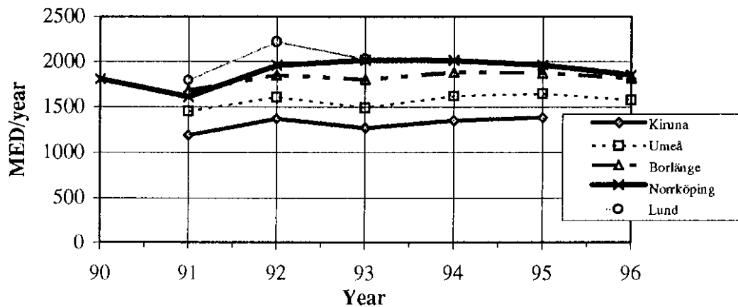
Figure 5.2 Yearly values from the five stations of the Swedish network. Unit: MED/year. MED= Minimum Erythral Dose corresponding to 210 \text{ Jm}^{-2} CIE-weighted irradiance, WMO-STUK 1995 scale.
